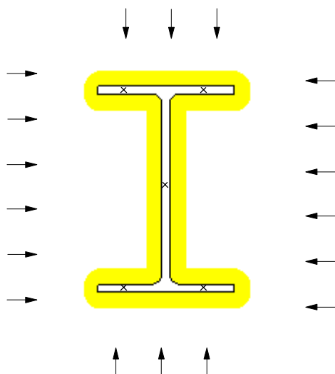
Figure 6.1 The setup of the SP-test with placing of thermocouples marked with X.
