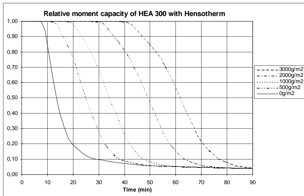
Figure 10.3 Relative moment capacity of HEA 300 with Hensotherm.
