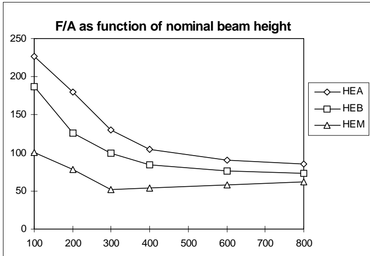
Figure 9.2a F/A as function of nominal beam height ( m^{-1} ).
