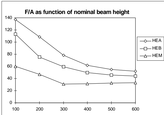
Figure 8.2a F/A as function of nominal beam height (m -1 ).
