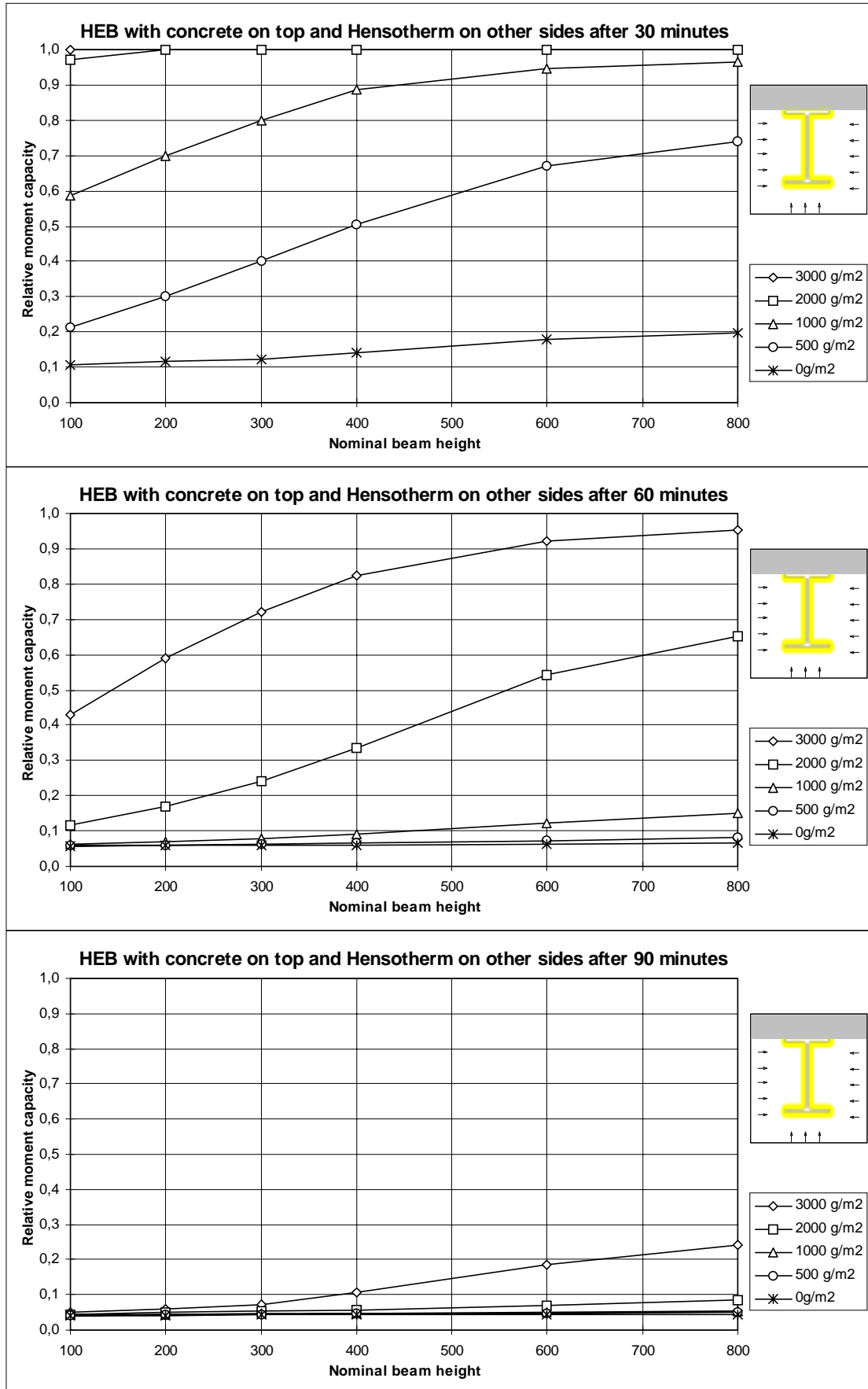
Figure 9.5 Relative moment capacity of HEB-beams with concrete on top.
