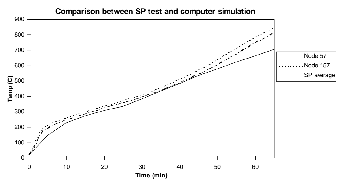
Figure 6.2 Comparison between SP test and computer simulation.
