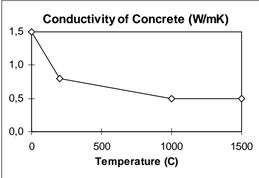
Figure 4.4 b) Conductivity of concrete.
