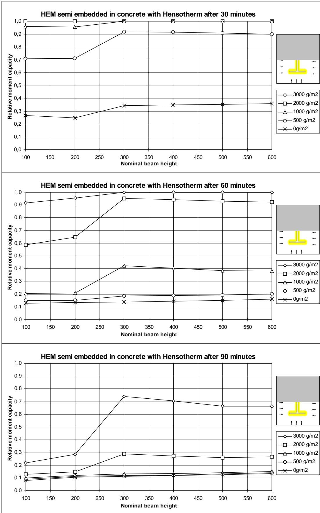
Figure 8.6 Relative moment capacity of HEM-beams semi embedded in concrete.
