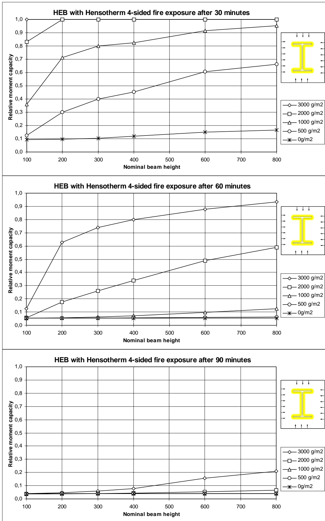
Figure 10.5 Relative moment capacity of HEB-beams with 4-sided fire exposure.
