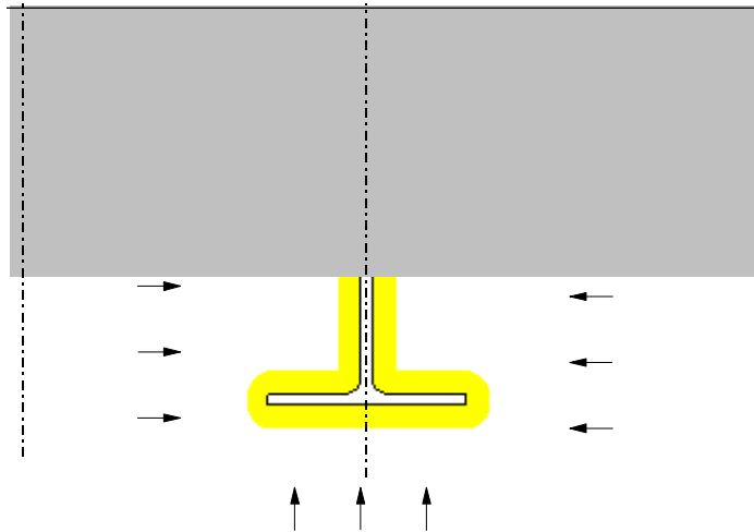
Figure 8.1 Steel beam semi embedded in concrete.
