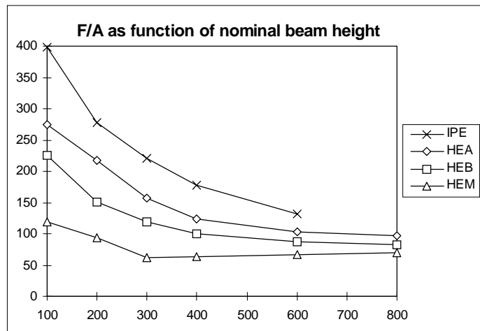
Figure 10.2a F/A as function of nominal beam height (m -1 ).
