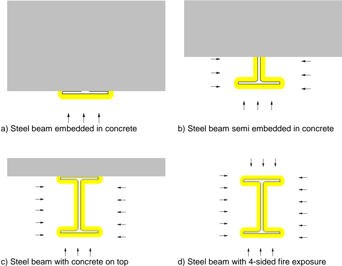
Figure 3.1 The four studied geometrical configurations.
