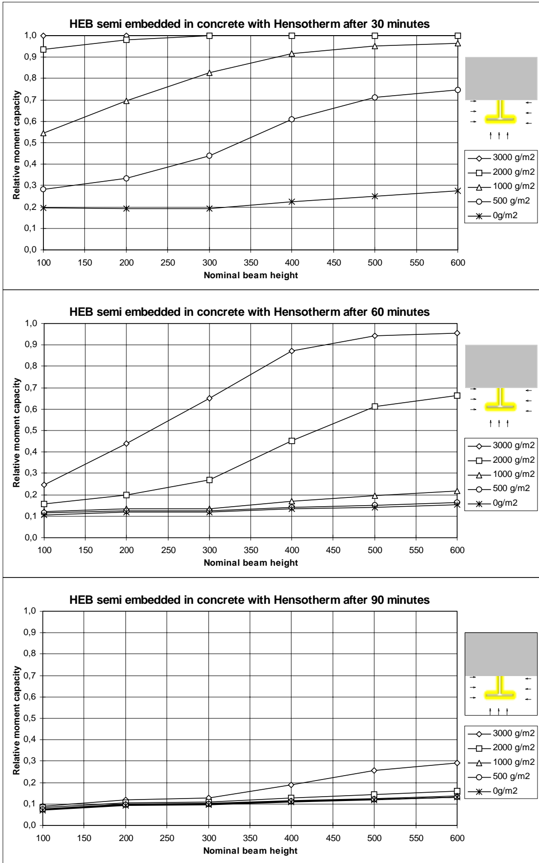
Figure 8.5 Relative moment capacity of HEB-beams semi embedded in concrete.
