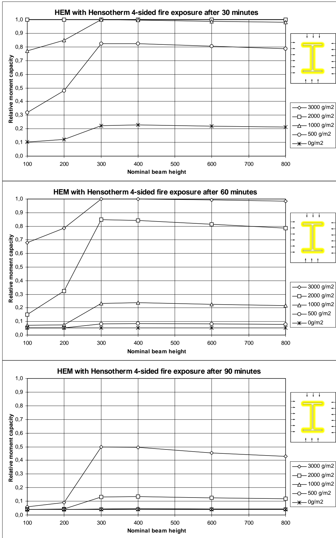
Figure 10.6 Relative moment capacity of HEM-beams with 4-sided fire exposure.
