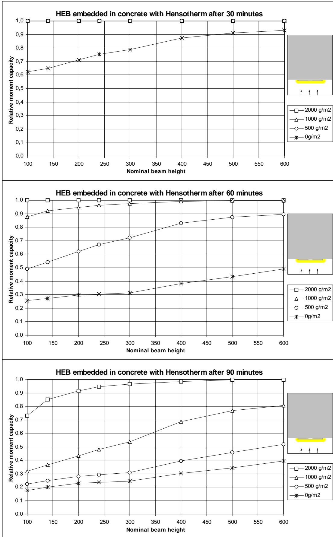
Figure 7.5 Relative moment capacity of HEB-beams embedded in concrete.
