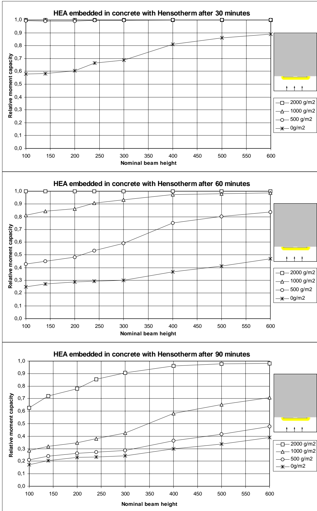
Figure 7.4 Relative moment capacity of HEA-beams embedded in concrete.
