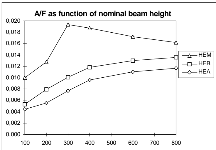
Figure 9.2b A/F as function of nominal beam height (m).
