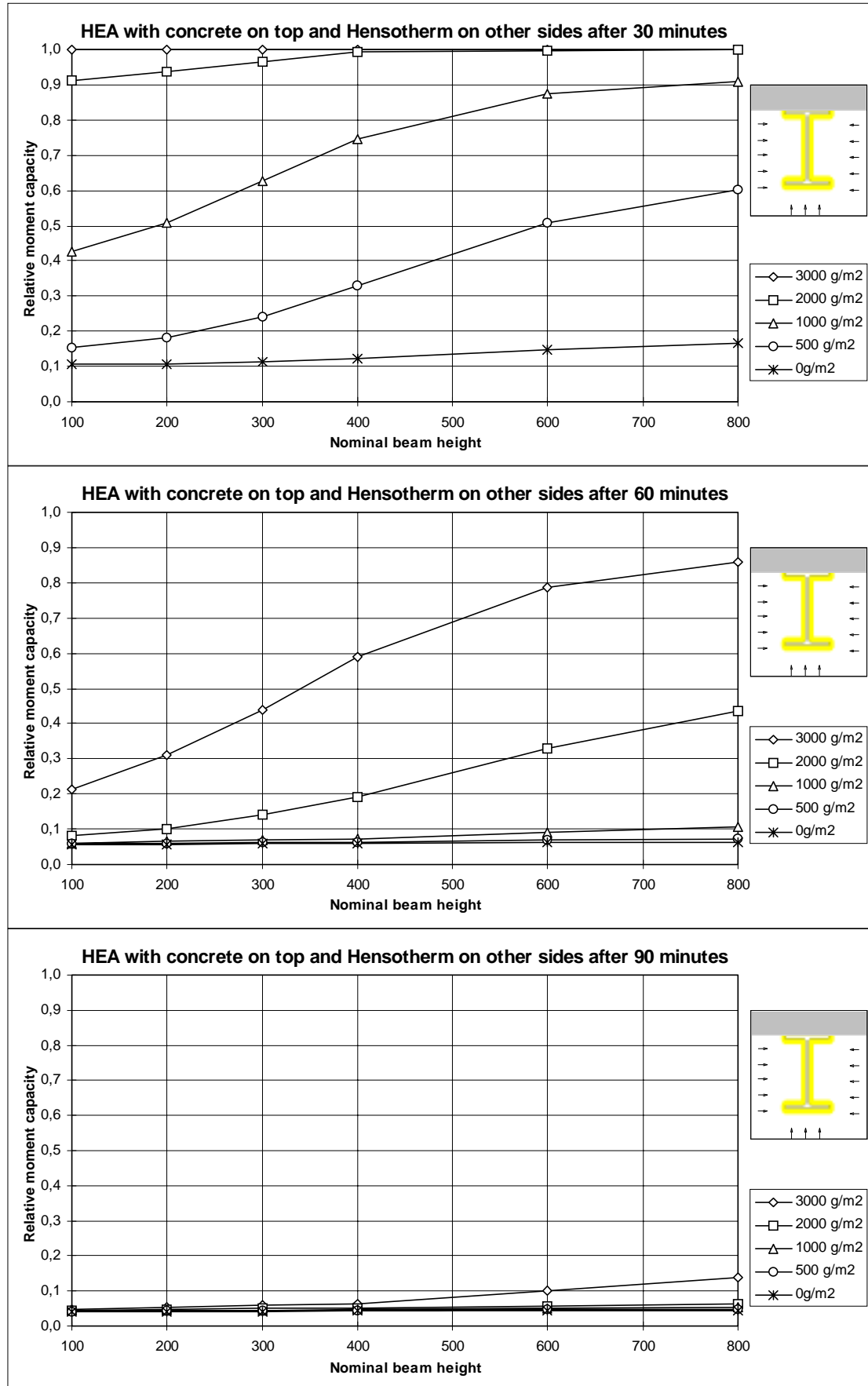
Figure 9.4 Relative moment capacity of HEA-beams with concrete on top.
