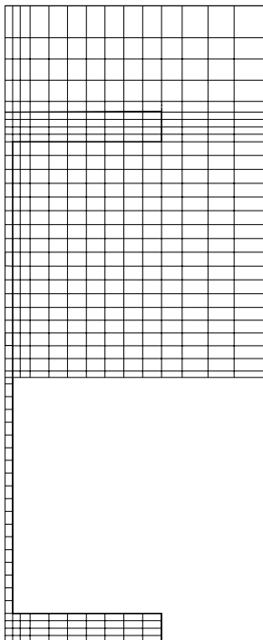
Figure 5.1 Grid of HEB 500 semi embedded in concrete.
