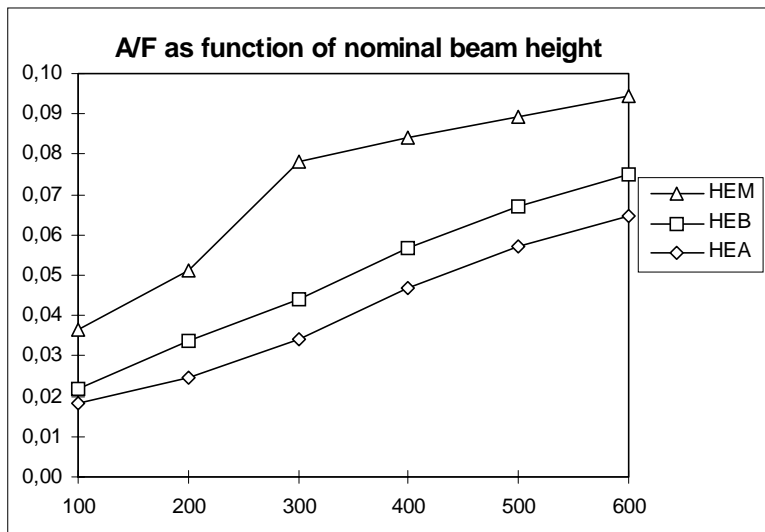
Figure 7.2b A/F as function of nominal beam height (m).
