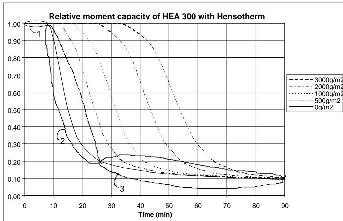
Figure 8.3 Relative moment capacity of HEA 300 with Hensotherm.
