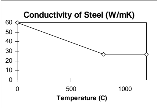
Figure 4.1 b) Thermal conductivity of steel.
