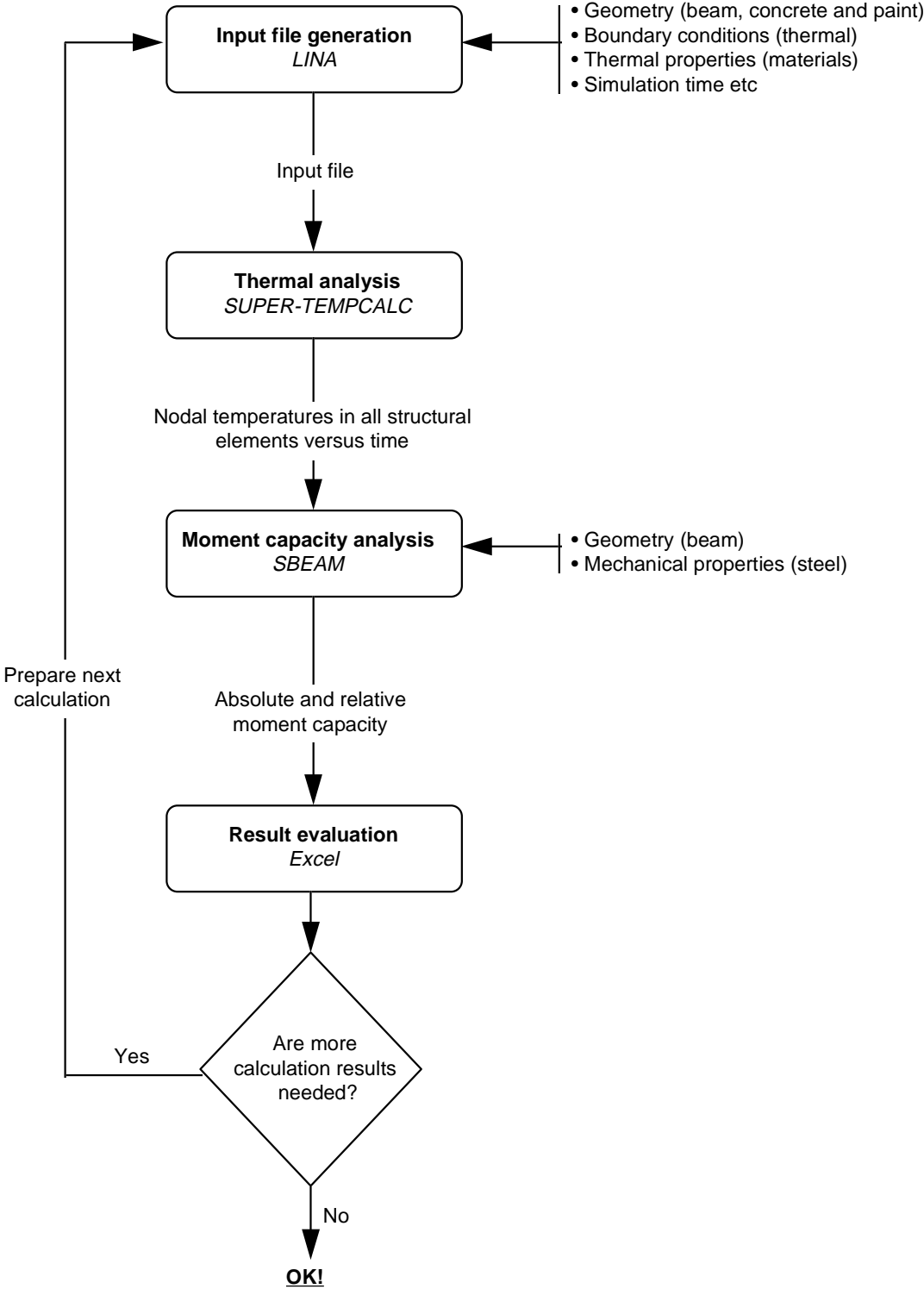
Figure 2.1 Method for calculation of moment capacity /18/.
