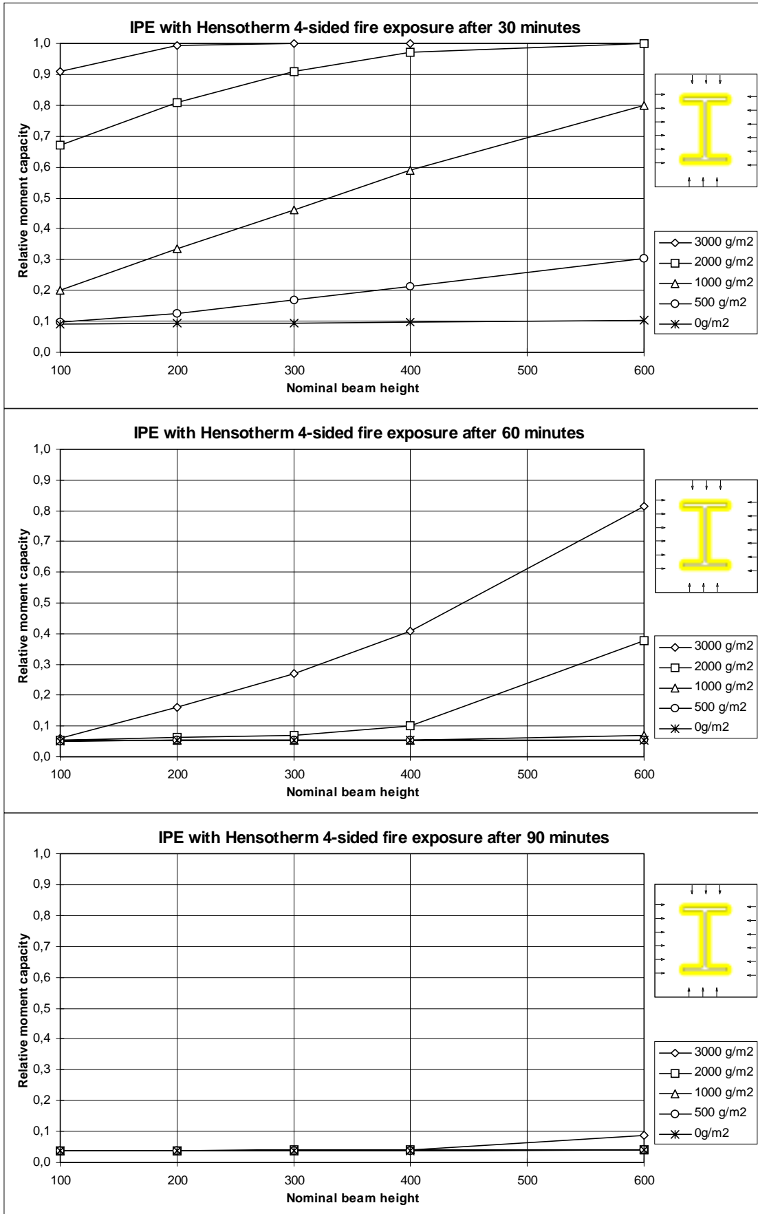
Figure 10.7 Relative moment capacity of IPE-beams with 4-sided fire exposure.
