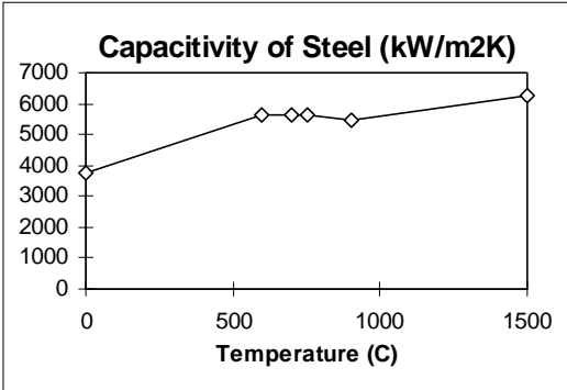
Figure 4.1 a) Thermal capacity of steel.
