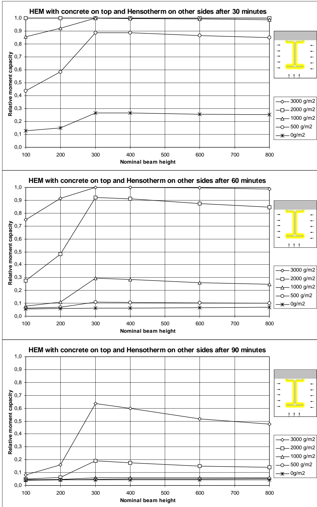
Figure 9.6 Relative moment capacity of HEM-beams with concrete on top.
