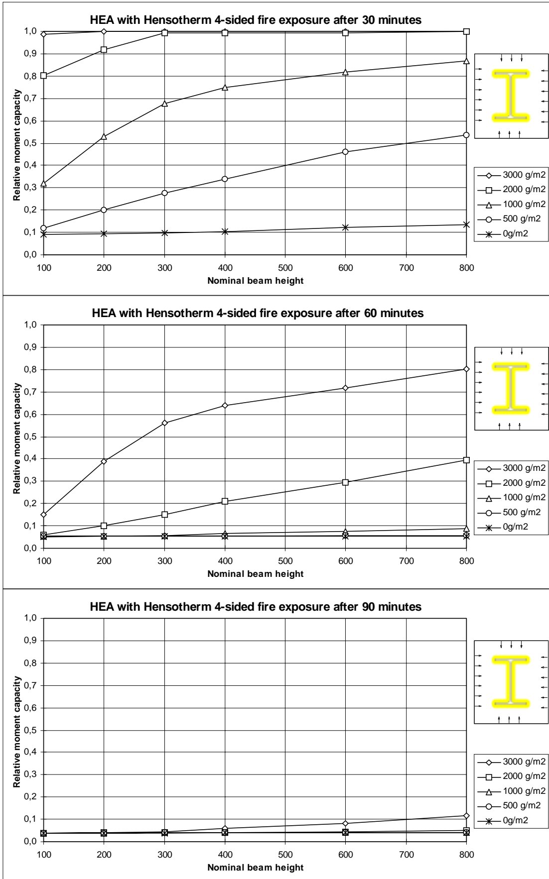
Figure 10.4 Relative moment capacity of HEA-beams with 4-sided fire exposure.
