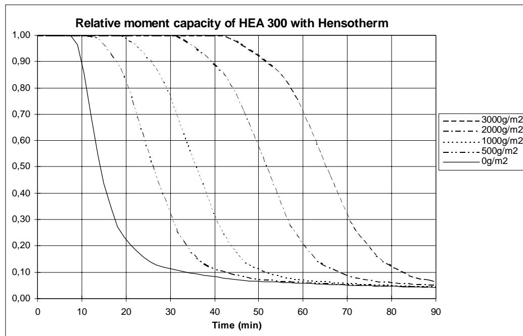
Figure 9.3 Relative moment capacity of HEA 300 with Hensotherm.
