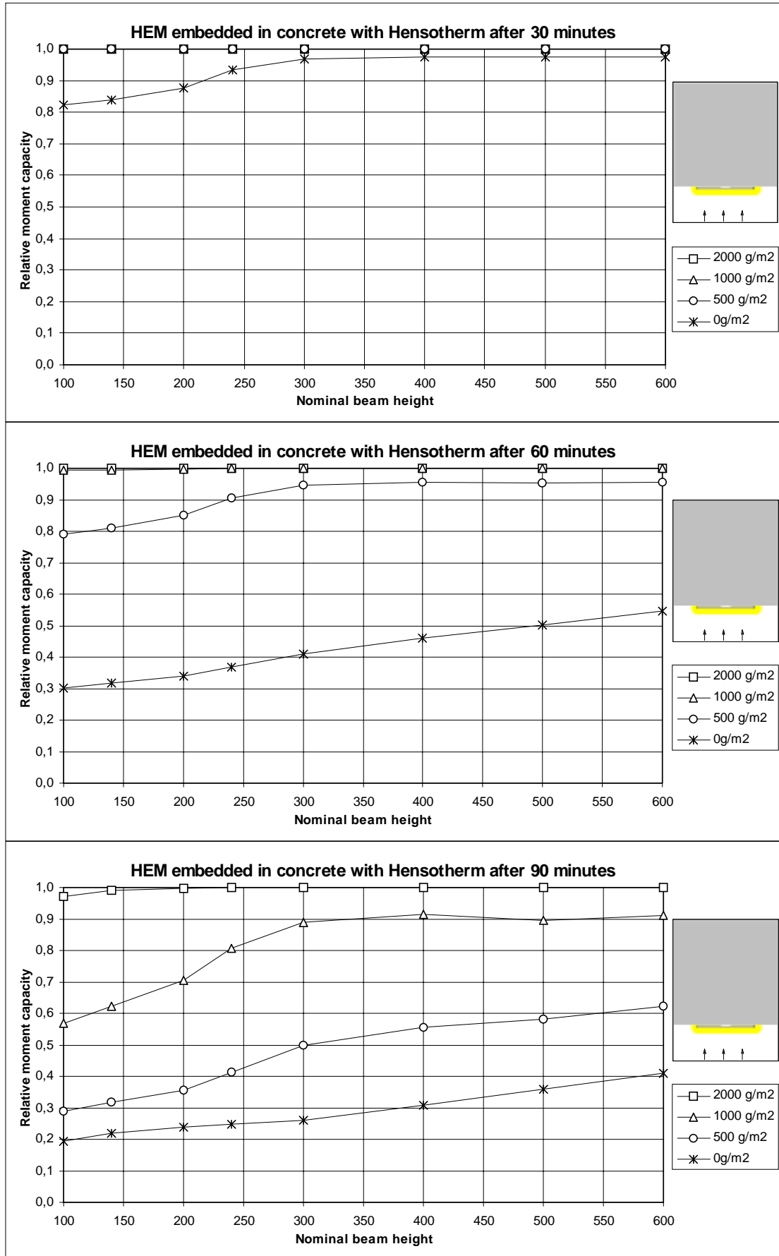
Figure 7.6 Relative moment capacity of HEM-beams embedded in concrete.
