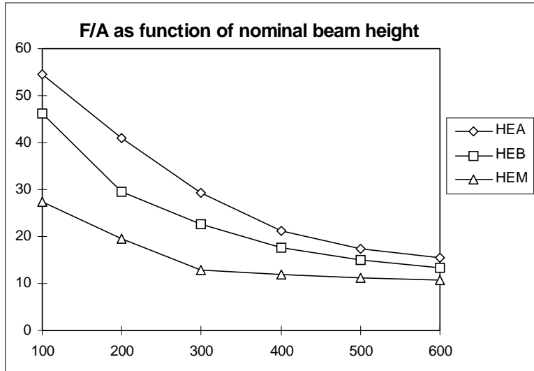
Figure 7.2a F/A as function of nominal beam height (m -1 ).
