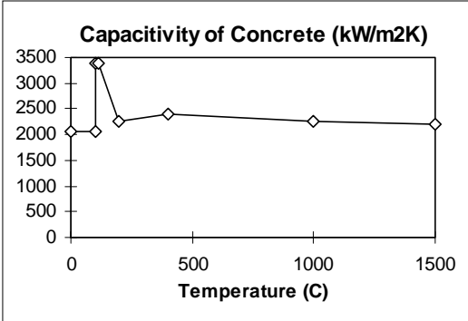
Figure 4.4 a) Capacity of concrete.
