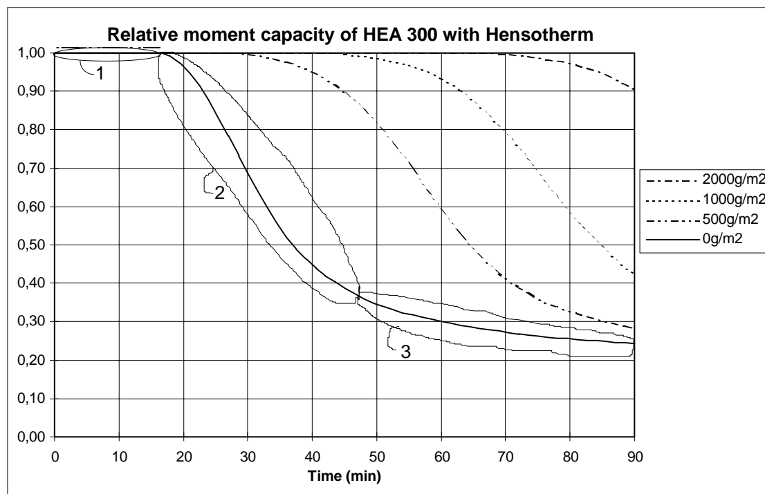
Figure 7.3 Relative moment capacity of HEA 300 with Hensotherm.
