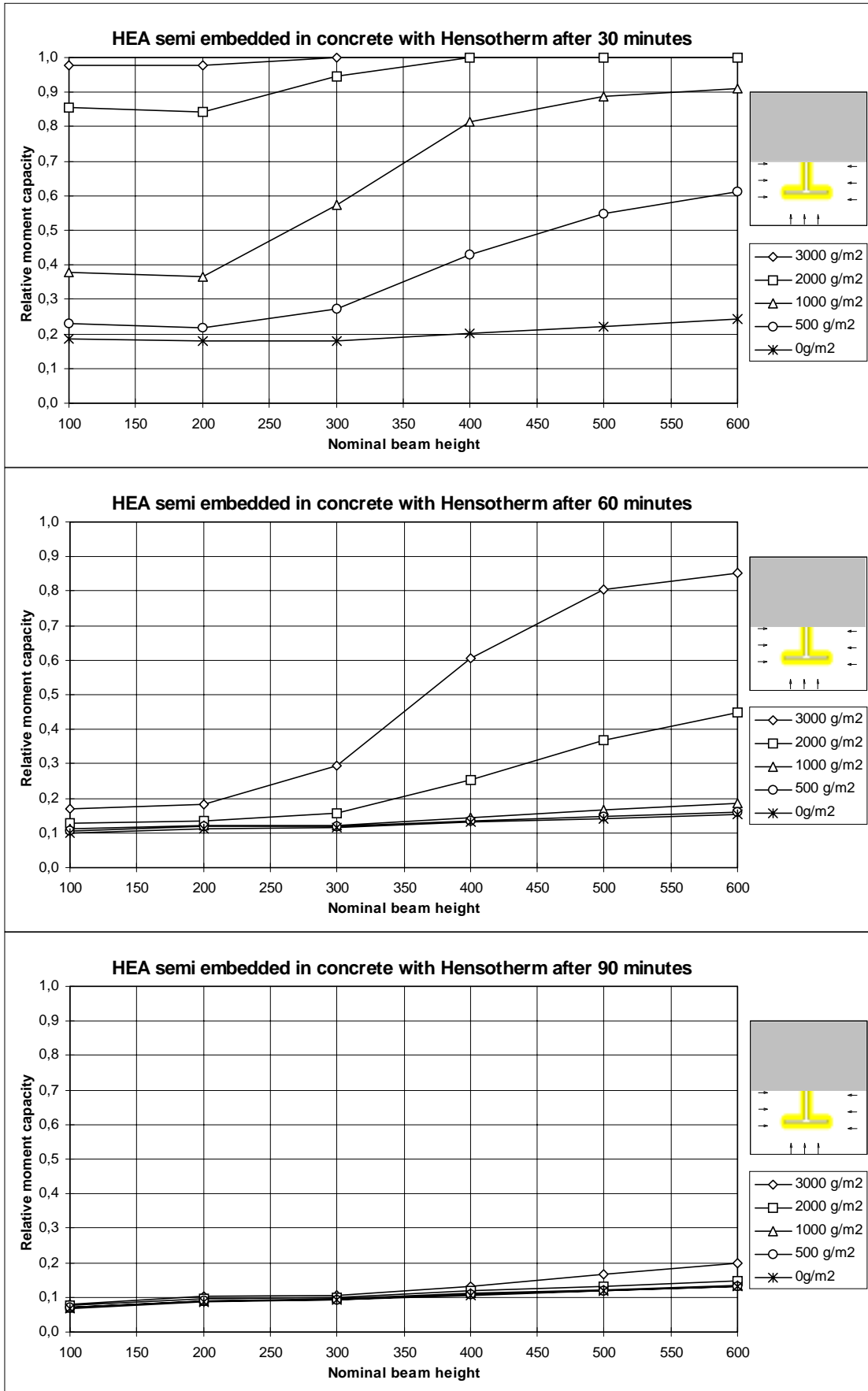
Figure 8.4 Relative moment capacity of HEA-beams semi embedded in concrete.
