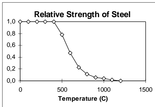
Figure 4.2 Relative strength of steel.
