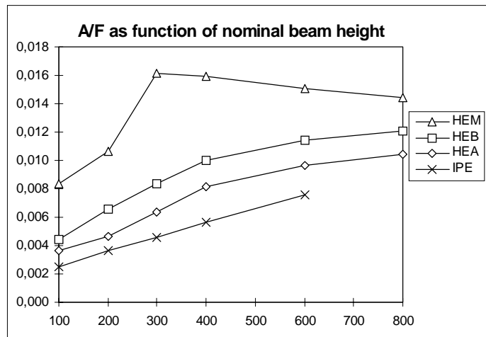
Figure 10.2b A/F as function of nominal beam height (m).
