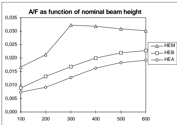
Figure 8.2b A/F as function of nominal beam height (m).
