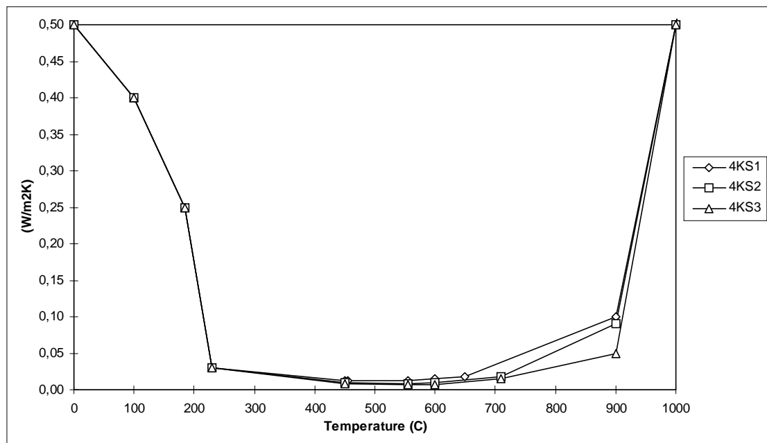
Figure 4.3 Thermal conductivity of Hensotherm.
