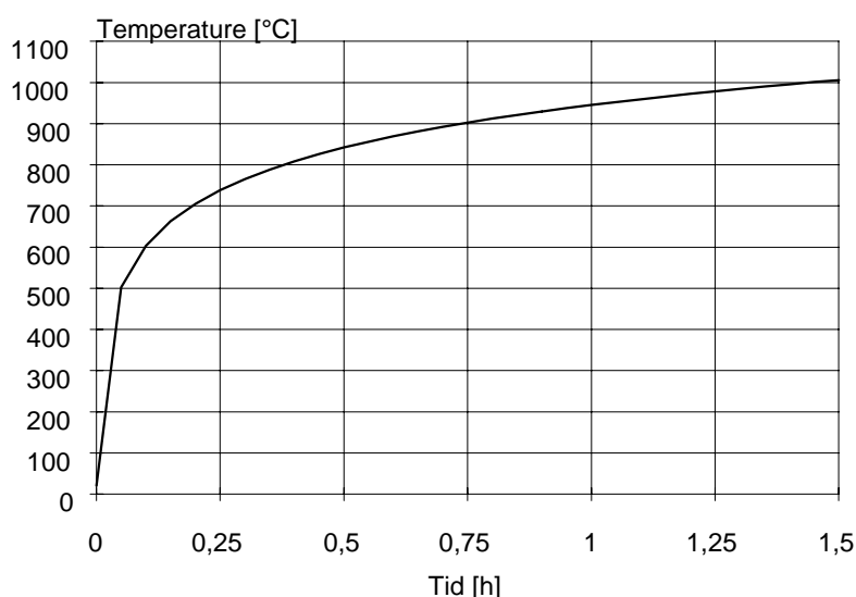
Figure 3.2 Temperature as function of time according to ISO 834.
