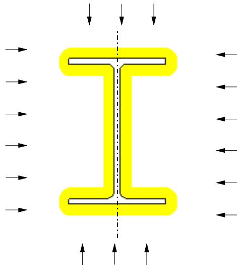
Figure 10.1 Steel beam with 4-sided fire exposure.
